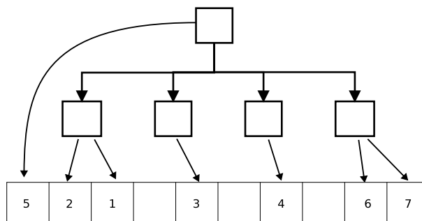
Figure 177: Quad trees as spatial acceleration structures
